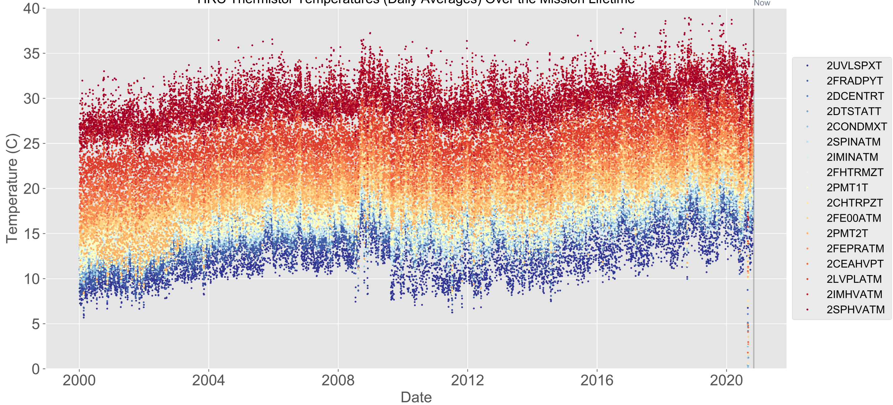
HRC Thermistor Temperatures (Daily Averages) Over the Mission Lifetime
