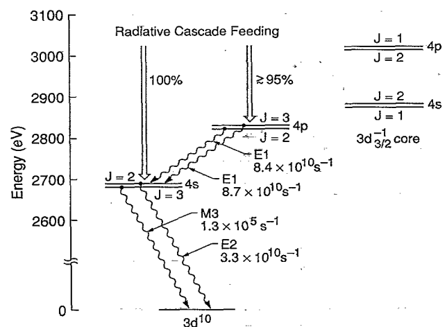
FIG. 1. Level diagram of nickel-like \text{U}^{64+} showing the lowest eight excited levels. Radiative decay rates are indicated for the four lowest levels, which have a 3d^5 3d^5 core. These levels are populated almost exclusively by radiative cascades from higher levels.
