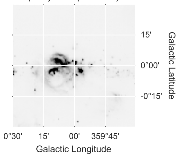
plt.style.use('seaborn')
