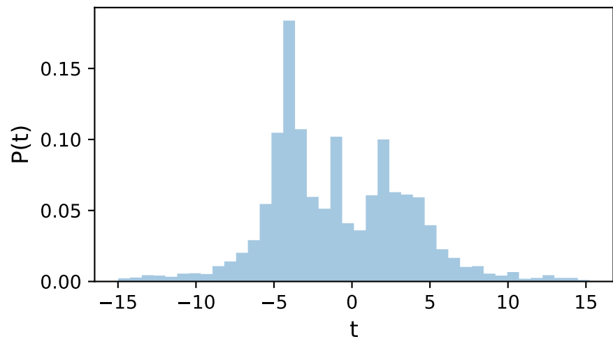
hist(t, bins="freedman")
