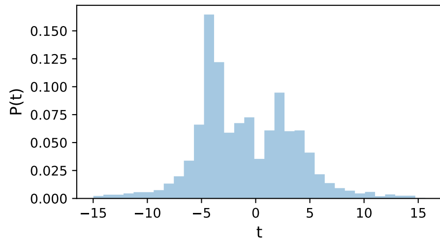
hist(t, bins="scott")
