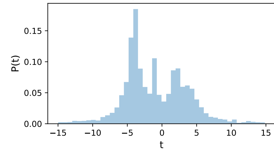
hist(t, bins="knuth")
