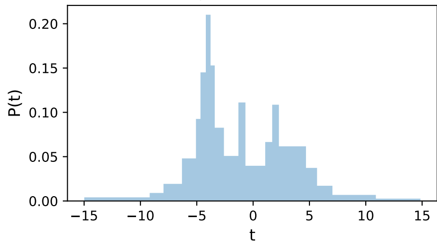
hist(t, bins="blocks")
