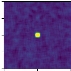
Box2DKernel
