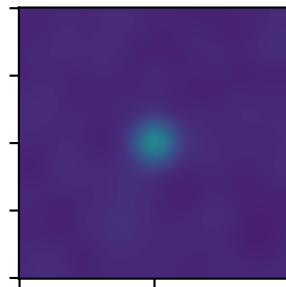
Gaussian2DKernel
