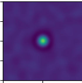
MexicanHat2DKernel
