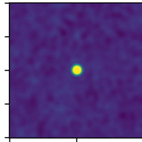
AiryDisk2DKernel
