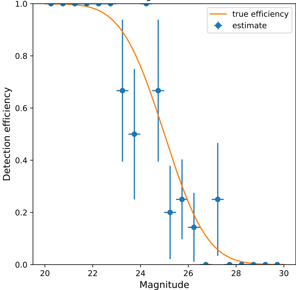
The Wald interval can give nonsensical uncertainties
