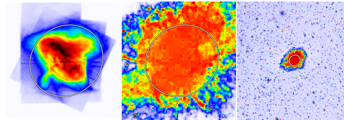
2MASS-J.hires.fits:
