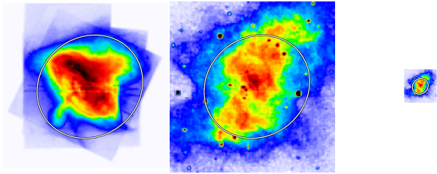
2MASS-K.hires.fits:
