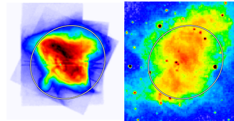
2MASS-J.hires.fits:
