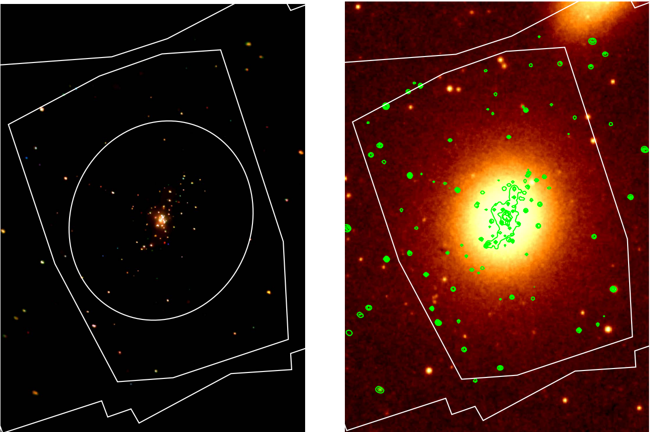
Fig. 1.— Top: An optical image of NGC 3379, with full band, adaptively smoothed, X-ray contours overlaid. Also shown is the outline of the total area covered by the ACIS-S3 chips, from the five separate observations, and the smaller region overlapped by all five of the pointings. Bottom: A ‘true color’ image of the galaxy, where red corresponds to 0.3–0.8 keV, green to 0.8–2.5 keV and blue to 2.5–8.0 keV. The D_{25} ellipse of this galaxy, the coverage from all observations and the overlapping region are also shown.
