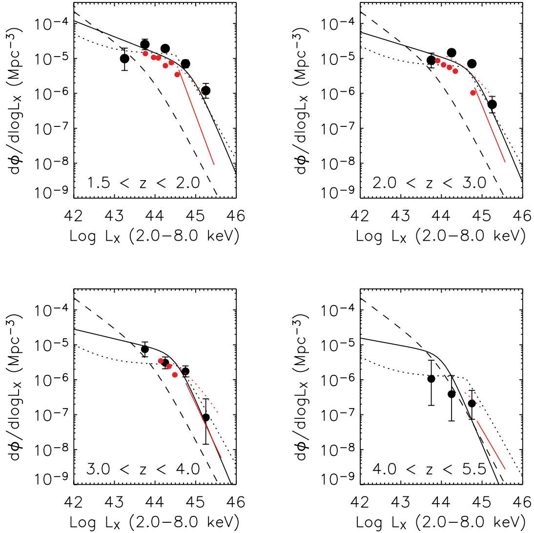
FIG. 15.—Comparison of the X-ray and optical luminosity functions at z > 1.5 . The black filled circles and lines are our data as shown in Fig. 9. The optical luminosity function is overplotted for the SDSS ( solid red line ; Richards et al. 2006), optically faint SDSS ( small red filled circles ; Jiang et al. 2006), and COMBO-17 ( dotted red line ; Wolf et al. 2003).
