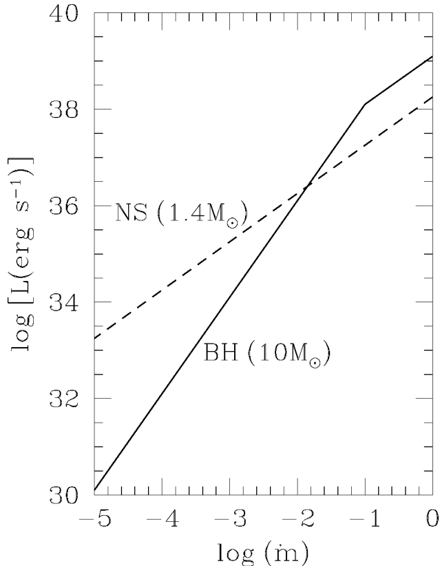
FIG. 1.—Expected variation of the luminosities of BH SXTs and NS SXTs as functions of the Eddington-scaled mass accretion rate \dot{m} (based on Fig. 11 of Narayan & Yi 1995). The solid line corresponds to a 10 M_{\odot} BH. For \dot{m} > 0.1 , the accretion is assumed to take place via a thin disk with the standard 10% efficiency, while for \dot{m} < 0.1 , the flow is assumed to be an ADAF with reduced efficiency. The dashed line corresponds to a NS SXT ( M_{\text{NS}} = 1.4 M_{\odot} ), for which the efficiency is taken to be 10% regardless of the mode of accretion. Since \dot{m} varies by a few orders of magnitude between outburst and quiescence, we expect BH SXTs to exhibit a substantially larger variation of L than NS SXTs. Fig. 2 confirms this prediction.
