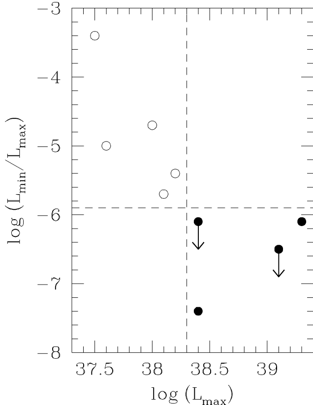
FIG. 2.—The outburst luminosities L_{\max} and luminosity ranges L_{\min}/L_{\max} of the NS SXTs (open circles) and BH SXTs (filled circles) listed in Table 2. Upper limits are indicated by arrows. We have left the BH SXT H1705–25 off the plot because the observation used to compute the upper limit on L_{\min} is more than an order of magnitude less sensitive than the observations of the other 4 BH SXTs (see Table 1). The vertical dashed line represents L_{\text{Edd}} for a 1.4 M_{\odot} NS. The horizontal dashed line is drawn to emphasize the point that every BH SXT has a lower value of L_{\min}/L_{\max} than every NS SXT. In the context of the ADAF model, this separation of BH SXTs and NS SXTs confirms that BH SXTs have horizons and NS SXTs do not.
