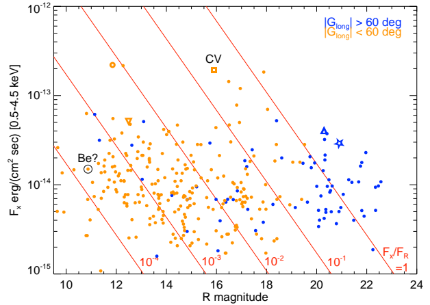
Fig. 7. Un-absorbed X-ray/optical flux vs. R (de-reddened) for initial sample of ChaMPlane sources inside vs. outside \ell = 60^\circ .
