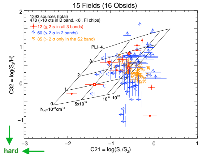
Fig. 3. Source X-ray colors and limits vs. PL models and N_H . Reduced source counts from 1393 total due to restriction \leq 6' (from center) and separate detections in individual bands. Bands are: S1=0.3–1.2keV, S2=1.2–2.5keV, H=2.5–8keV, B=0.3–8keV.
