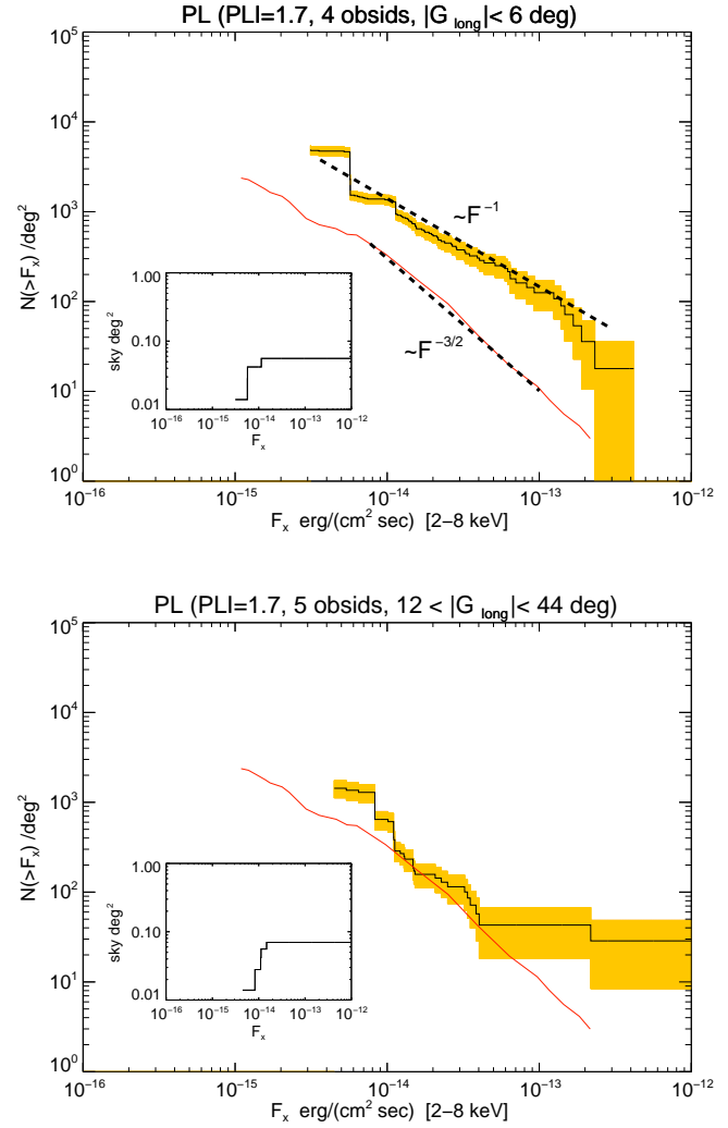
Fig. 2. Preliminary ChaMPPlane LogN-LogS and error band for sources in central ( \lesssim 4' ) Chandra fields in galactic longitude ranges shown compared with high latitude AGN counts.
